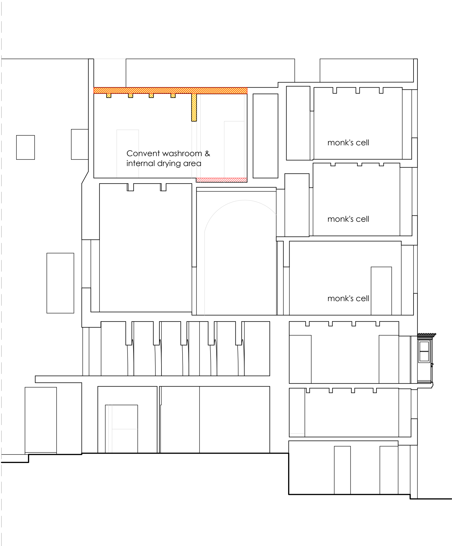
1 Section AA pre 1967, proposed changes marked
