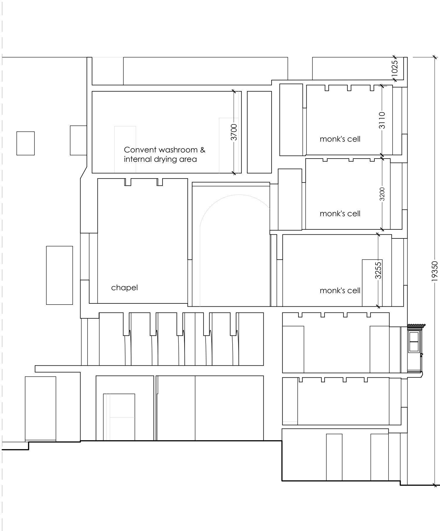
2 Section AA as proposed
